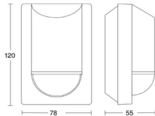
Dimensions (mm)
